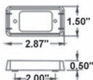
vsm9361 Black ABS Surface Mount Bracket
